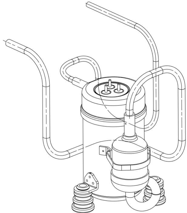
FIGURE 4: MESA single cylinder tubing suction loop
