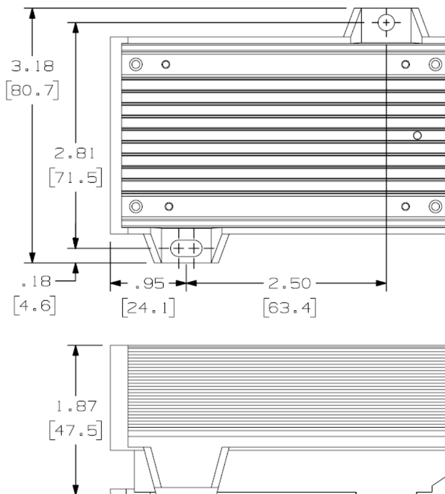
FIGURE 6: MESA controller dimensions in inches [mm]
