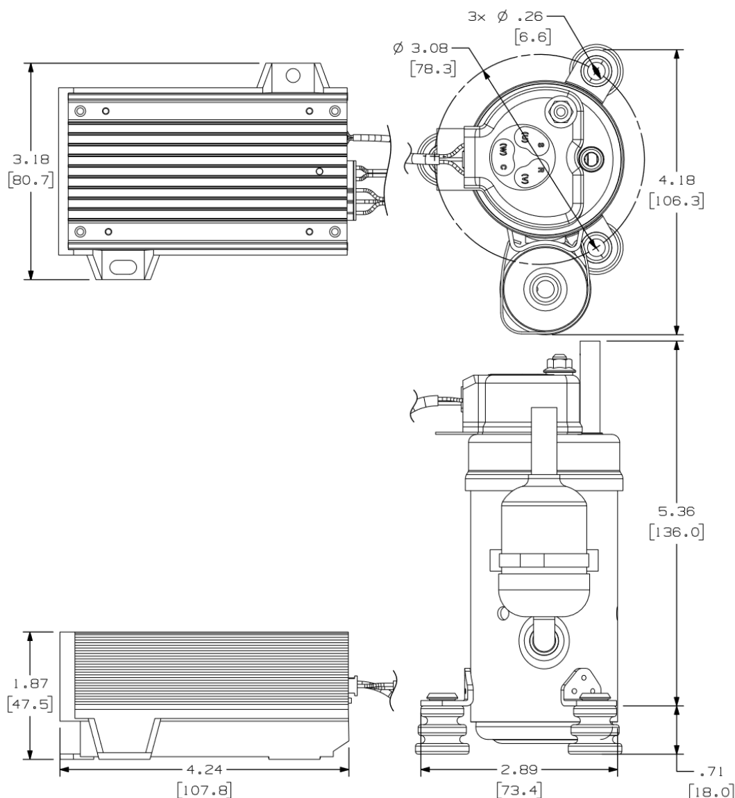
FIGURE 1: MESA twin cylinder inches [mm]
