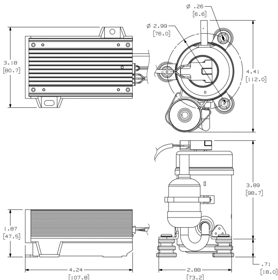
FIGURE 2: MESA single cylinder dimensions in inches [mm]
