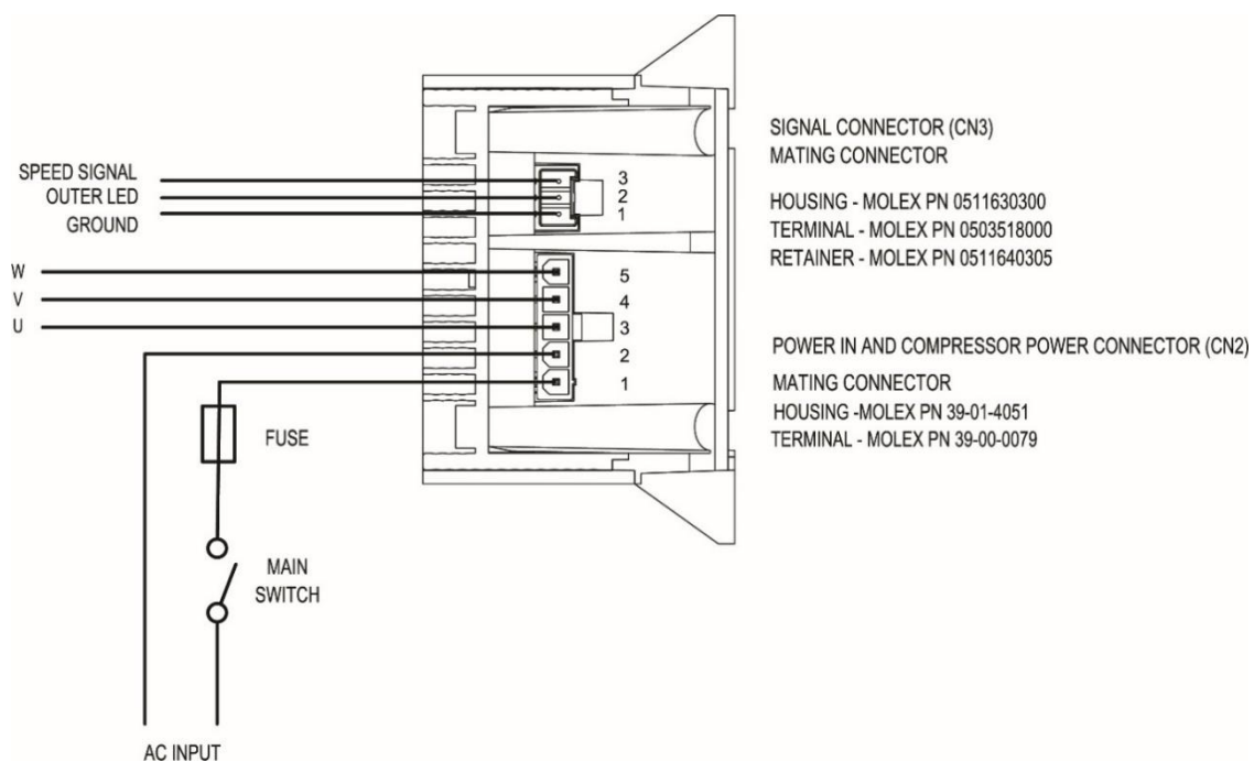
FIGURE 7: MESA wiring diagram
