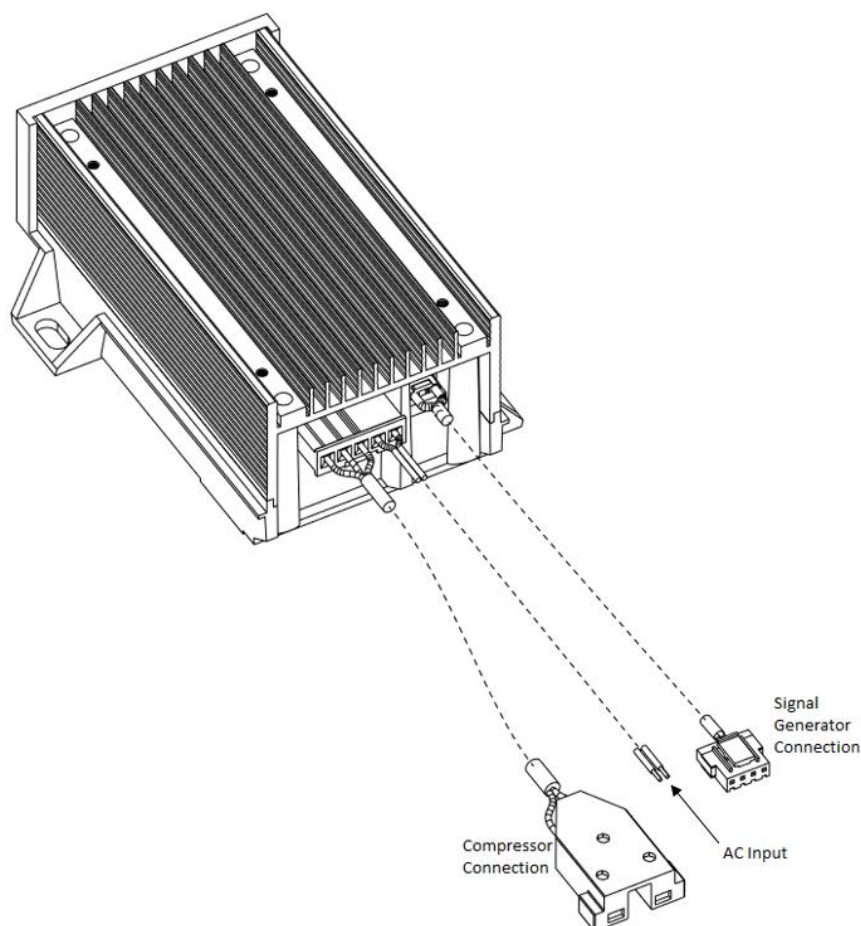
FIGURE 5: MESA controller with wires
